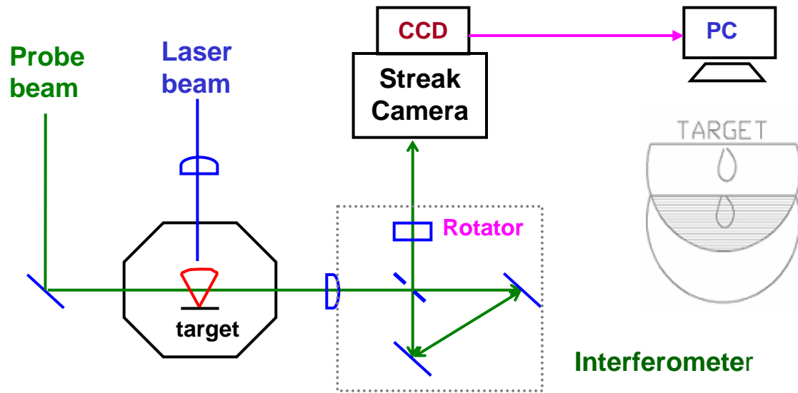
S-20 Optical streak camera
